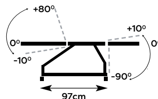
SUN-PHLEB2 Fixed Height Phlebotomy Chair with 4 locking castors
