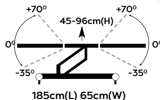
SUN-FVHC-3E 3 Section electric couch with powered height, head & foot section
