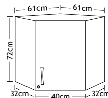
Sun-WU4 Corner Wall Cabinet
