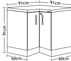
Sun-BU7 L-Shaped Corner Base Cabinet
