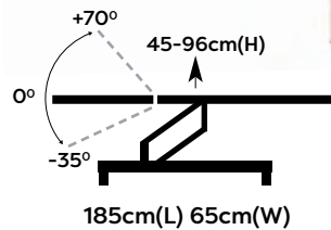
SUN-FECO2E Fusion 2 section electric couch
